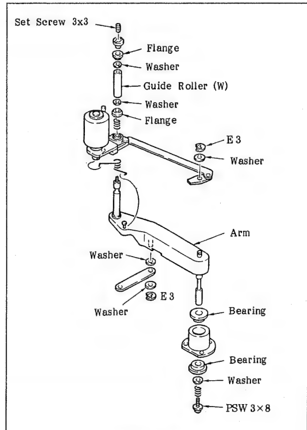
Fig. 6-113 Replacing the Arm
